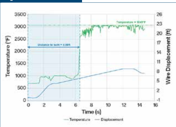
Temperature and level measurement marked-up to show how the distance to the steel bath and temperature values are determined.
