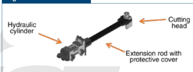
Model of the cored wire cutter installed at NSHC.
