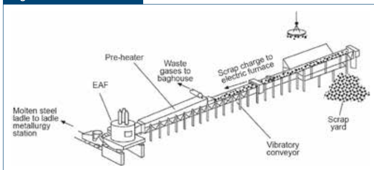
Overview of an electric arc furnace (EAF) with Consteel. 2
