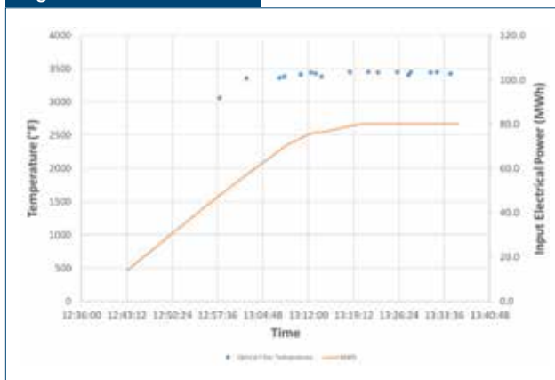
Temperature measurements from hot heat, Heat 607540.
