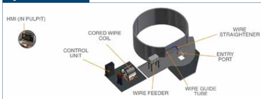
CoreTemp on-demand measurement system components. Note: The model of a person is only shown for the purposes of providing scale to the image.
