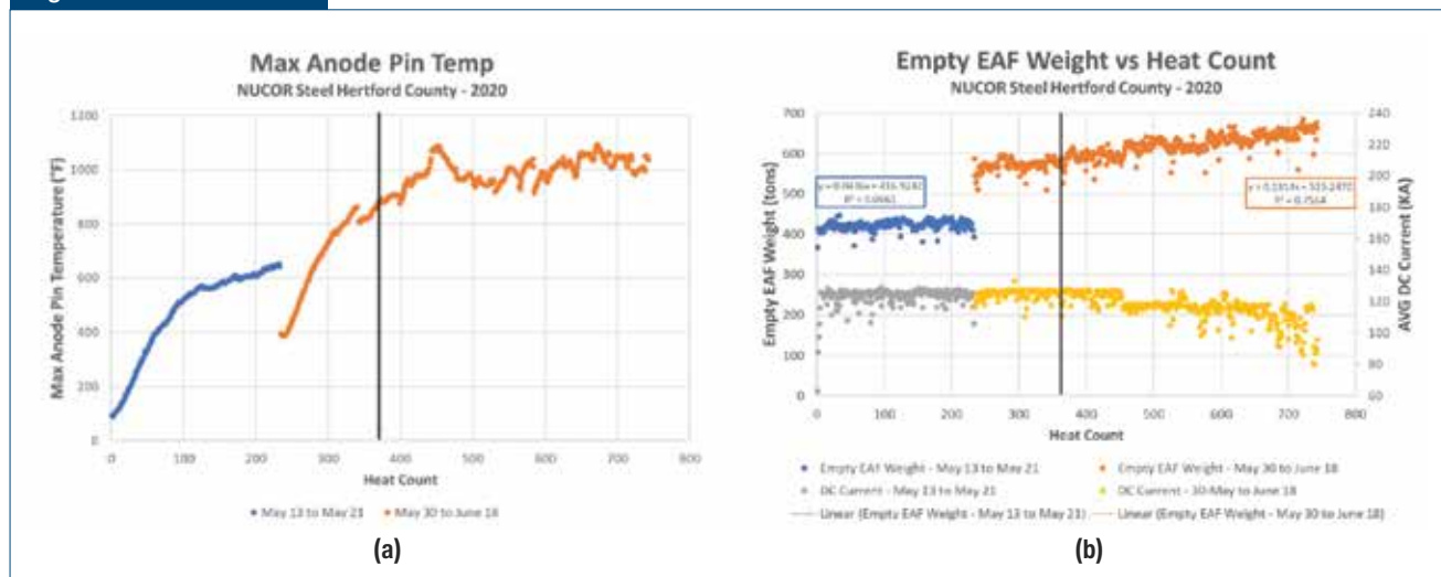
Plot of maximum anode pin temperature by heat count (a) and plot of empty EAF weight (heel weight inference) and average DC current by heat count (b).
